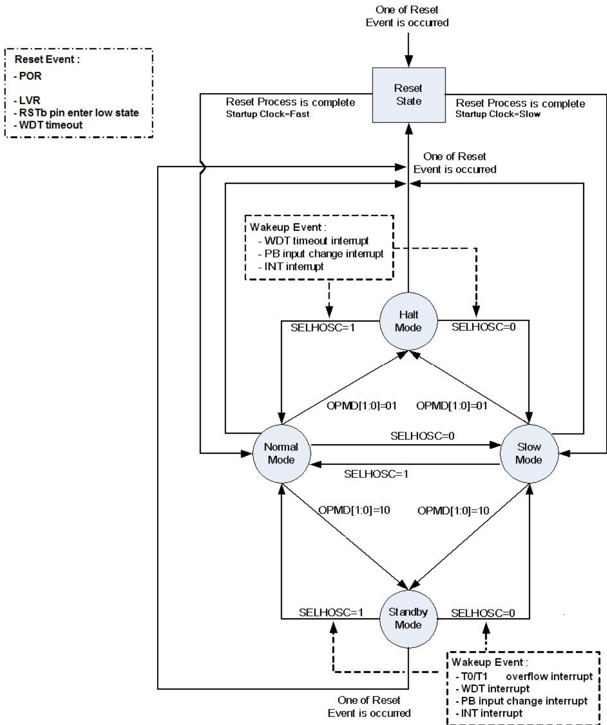
Figure 18 Four Operating Modes
