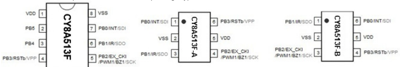
Figure 1 Package pin assignment
