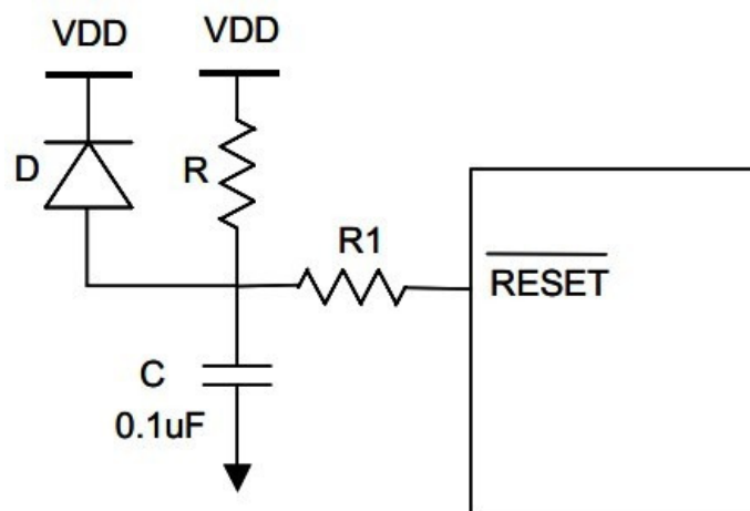
Figure 20 Block Diagram of Reset Application
