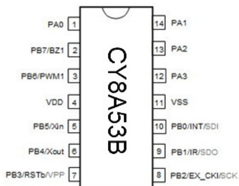
Figure 1 Package pin assignment
