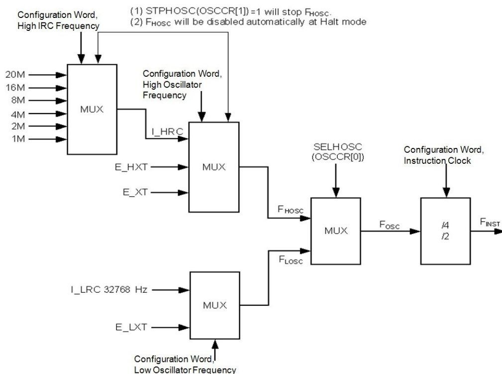
Figure 18 Oscillation Configuration of CY8A53B
