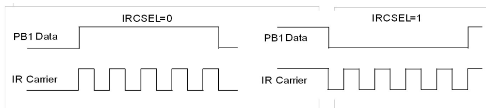
Figure 17 Polarity of IR Carrier vs. Output Data
