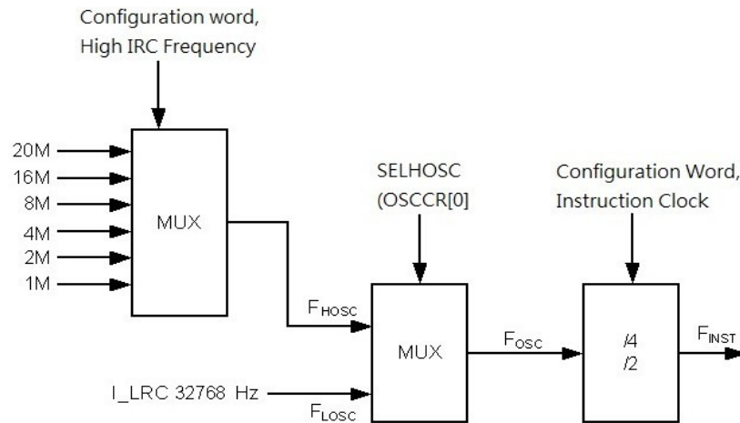
Figure 19 Oscillation Configuration of CY8AE513D
