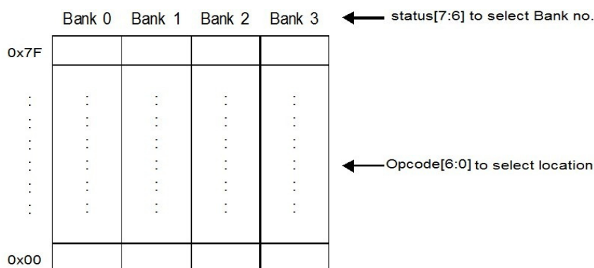
Figure 4 Direct Addressing Mode of Data Memory Access
