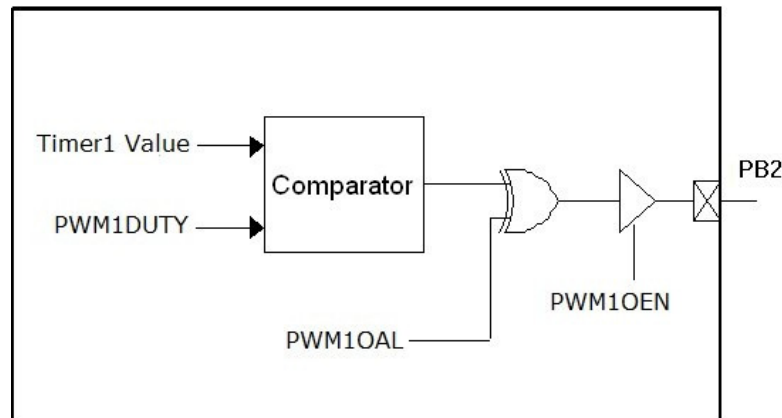
Figure 13 PWM1 Block Diagram
