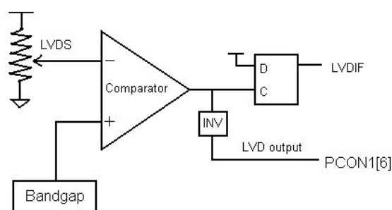
Figure 30 LVD block
