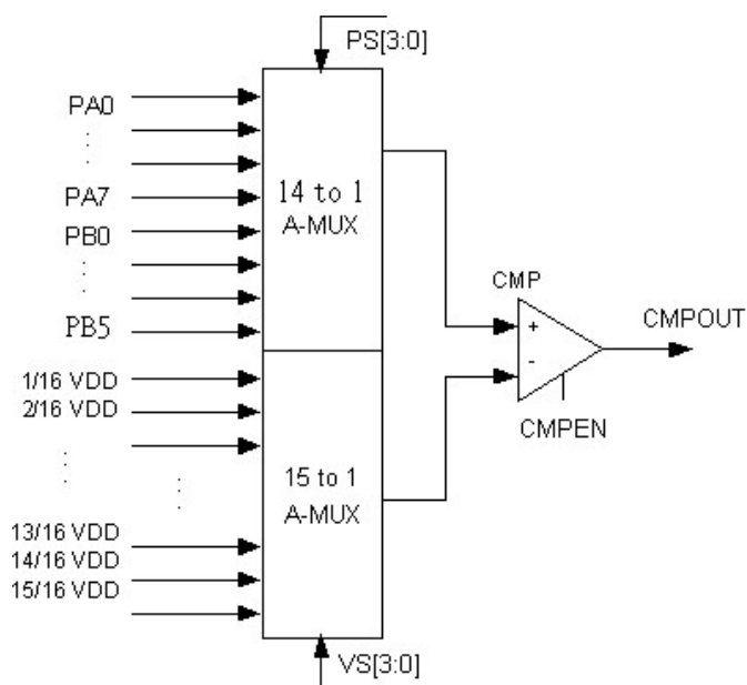
Figure 31 Comparator P2V mode block diagram
