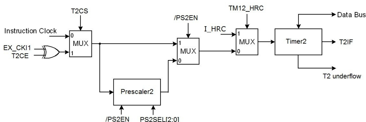
Figure 20 Block Diagram of Timer2
