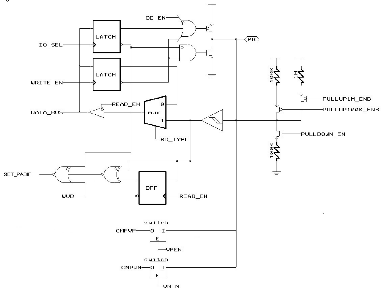
Figure 13 Block Diagram of PB2 & PB3
