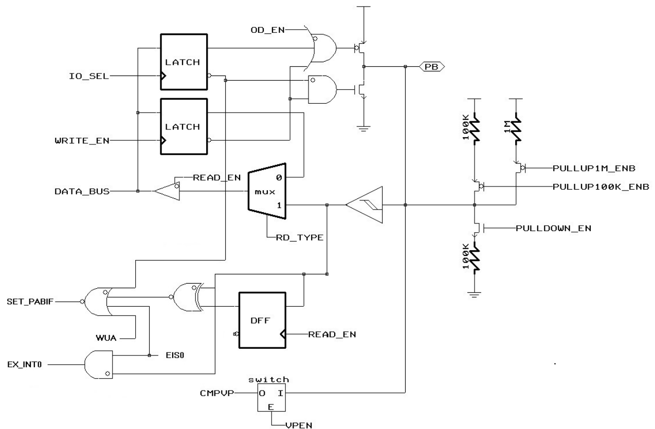
Figure 11 Block Diagram of PB0
