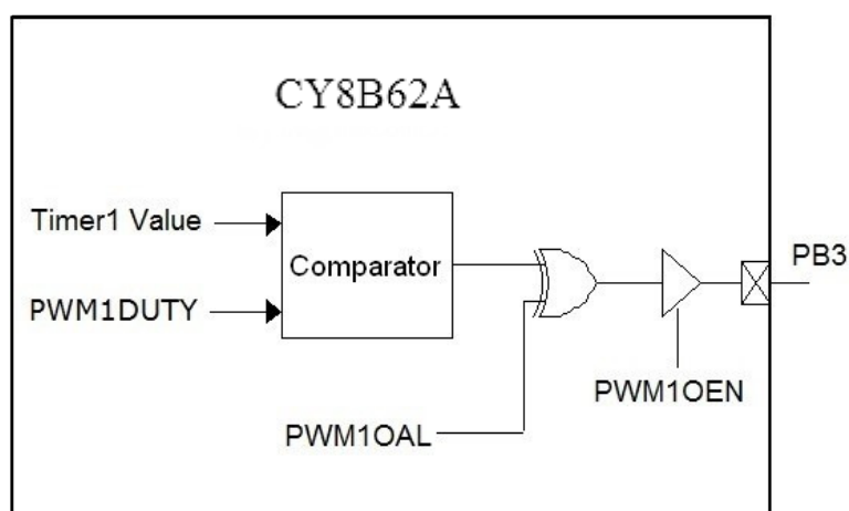
Figure 18 PWM1 Block Diagram
