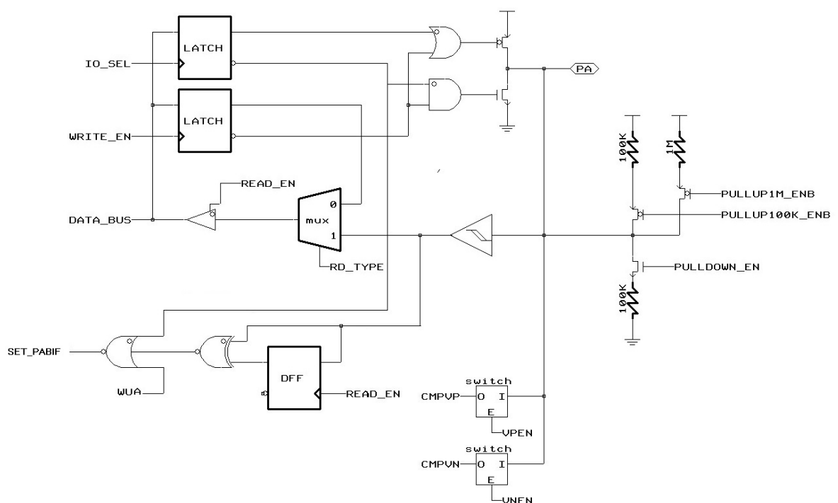
Figure 5 Block Diagram of PA2&PA0
