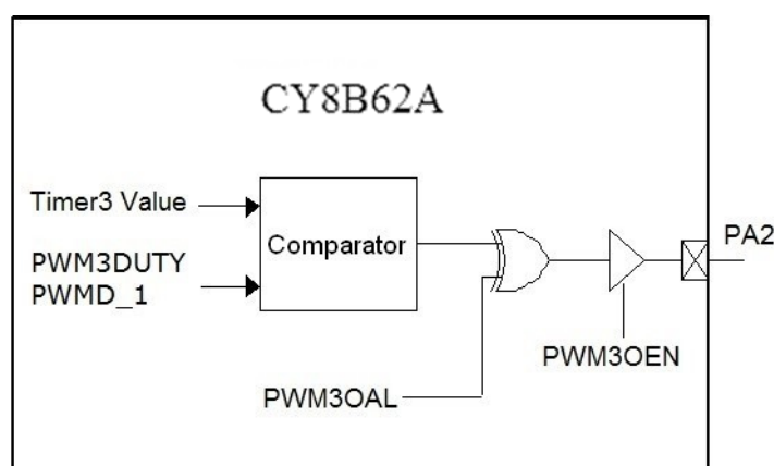
Figure 26 PWM3 Block Diagram
