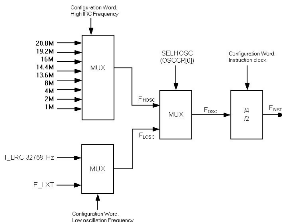
Figure 34 Oscillation Configuration of CY8B62A
