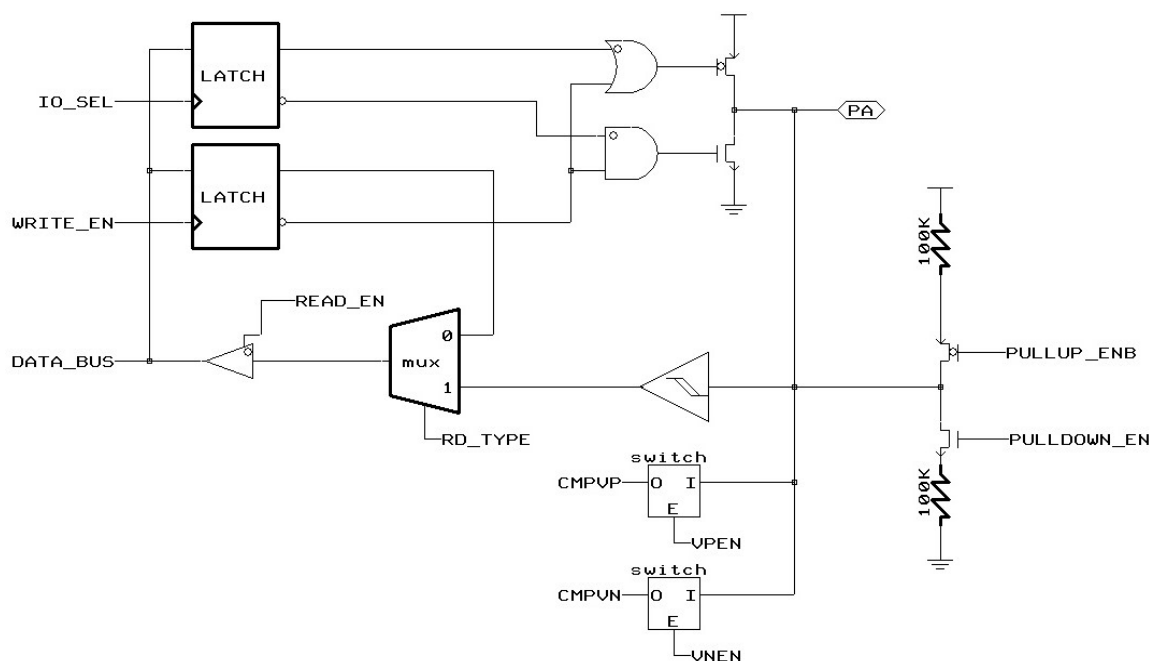
Figure 5 Block Diagram of PA[3:2]&PA0
