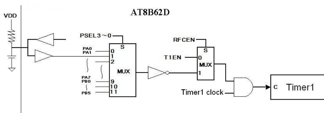
Figure 28 RFC Block Diagram
