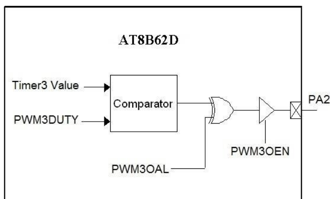
Figure 26 PWM3 Block Diagram
