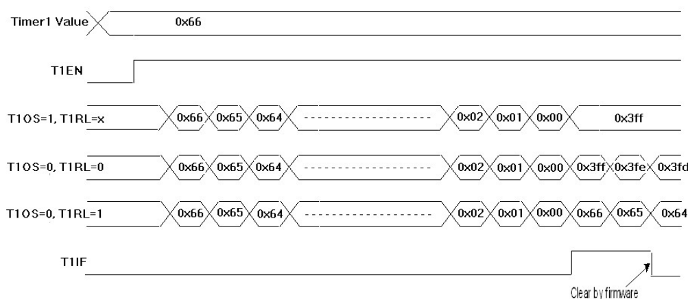
Figure 17 Timer1 Timing Chart
