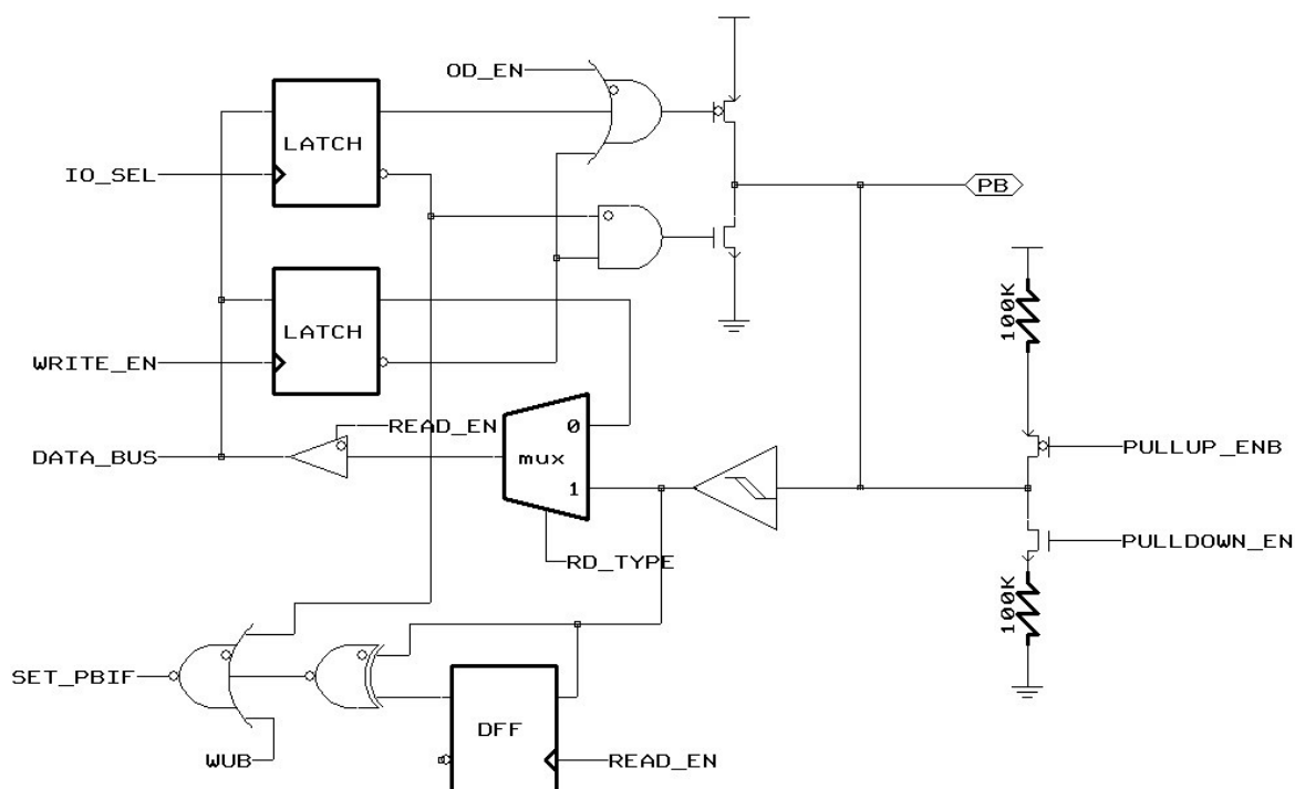
Figure 13 Block Diagram of PB3
