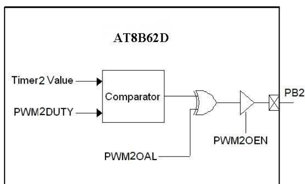
Figure 22 PWM2 Block Diagram
