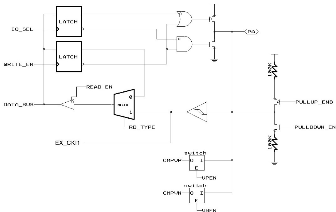
Figure 6 Block Diagram of PA1
