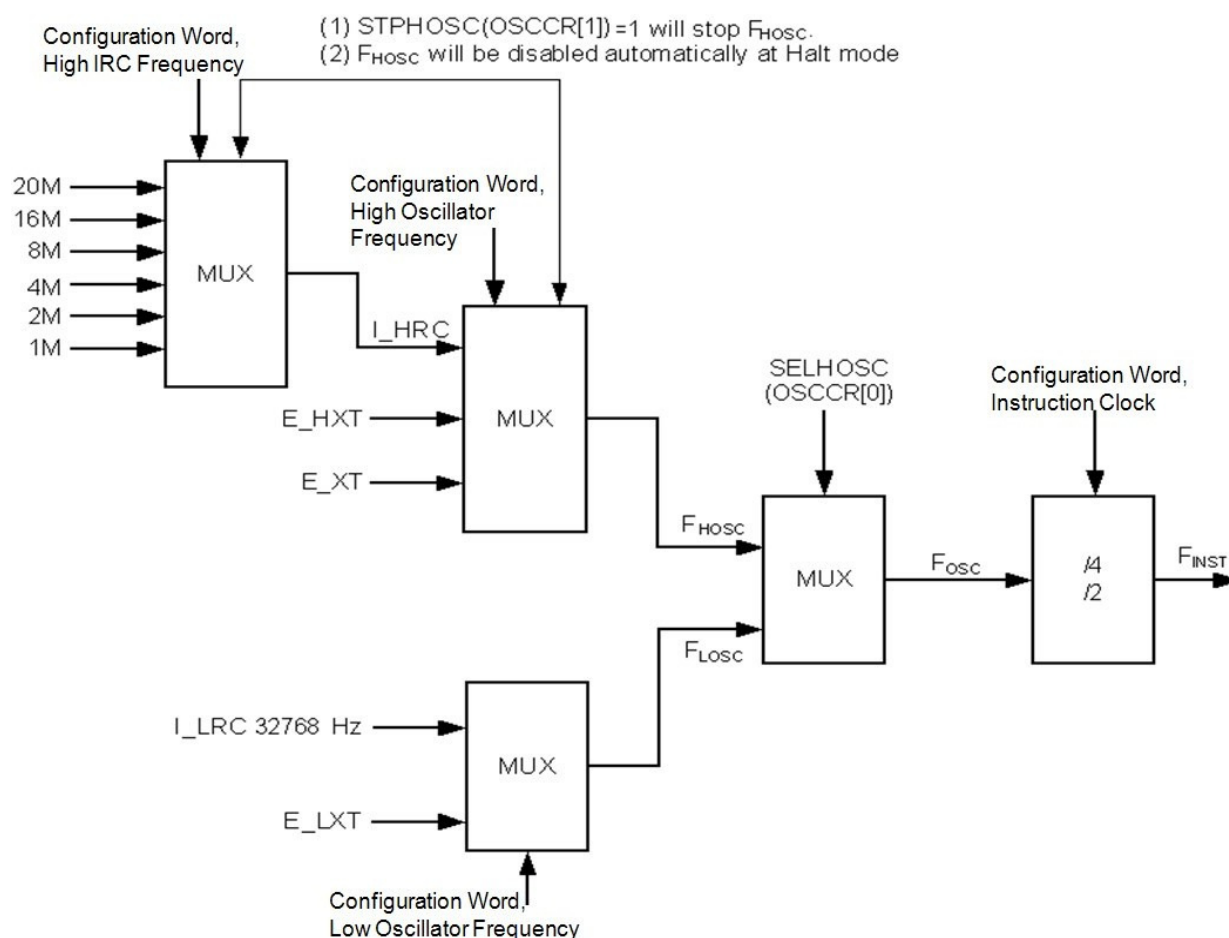
Figure 34 Oscillation Configuration of CY8B62D
