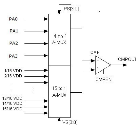
Figure 31 Comparator P2V mode block diagram
