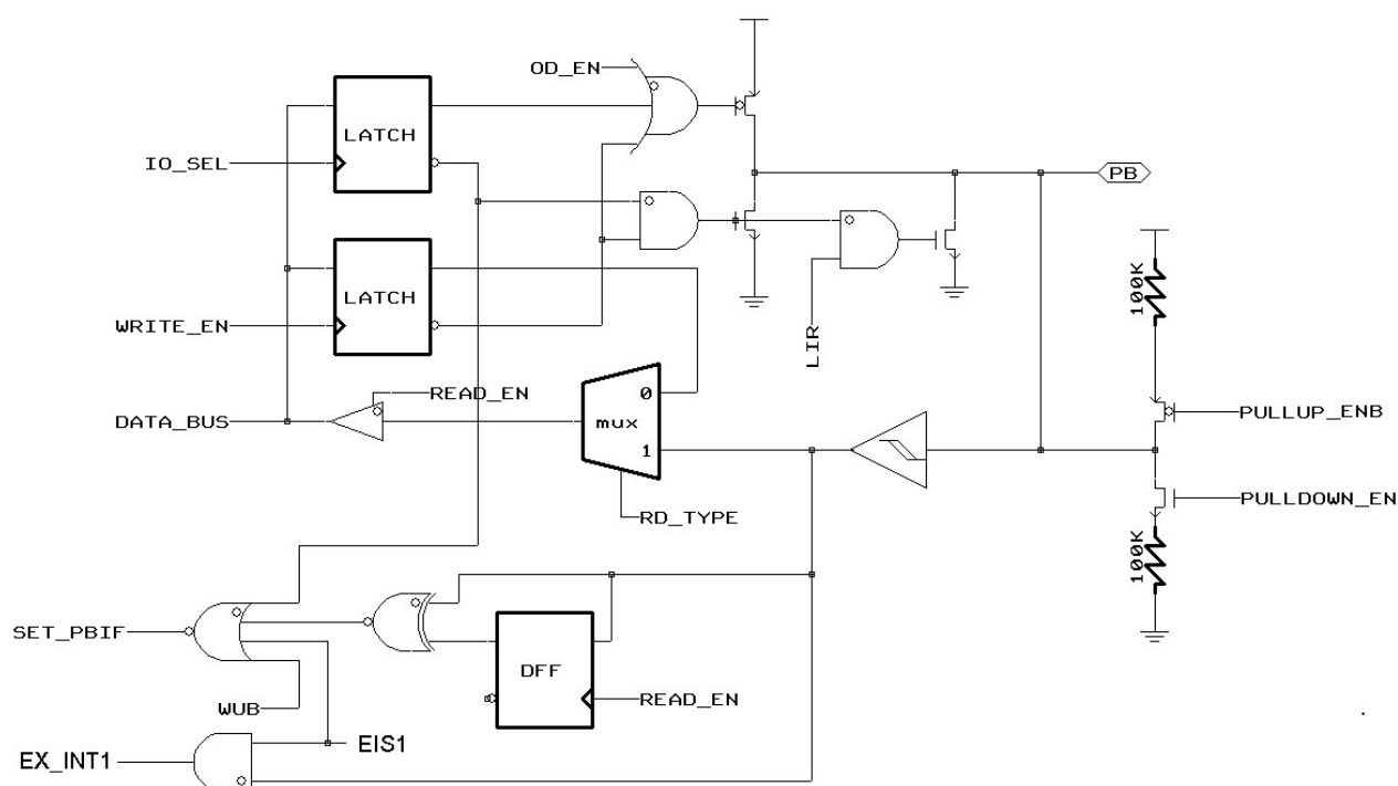
Figure 11 Block Diagram of PB1
