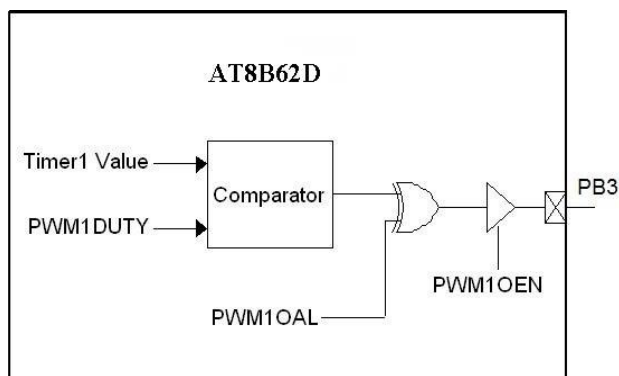
Figure 18 PWM1 Block Diagram
