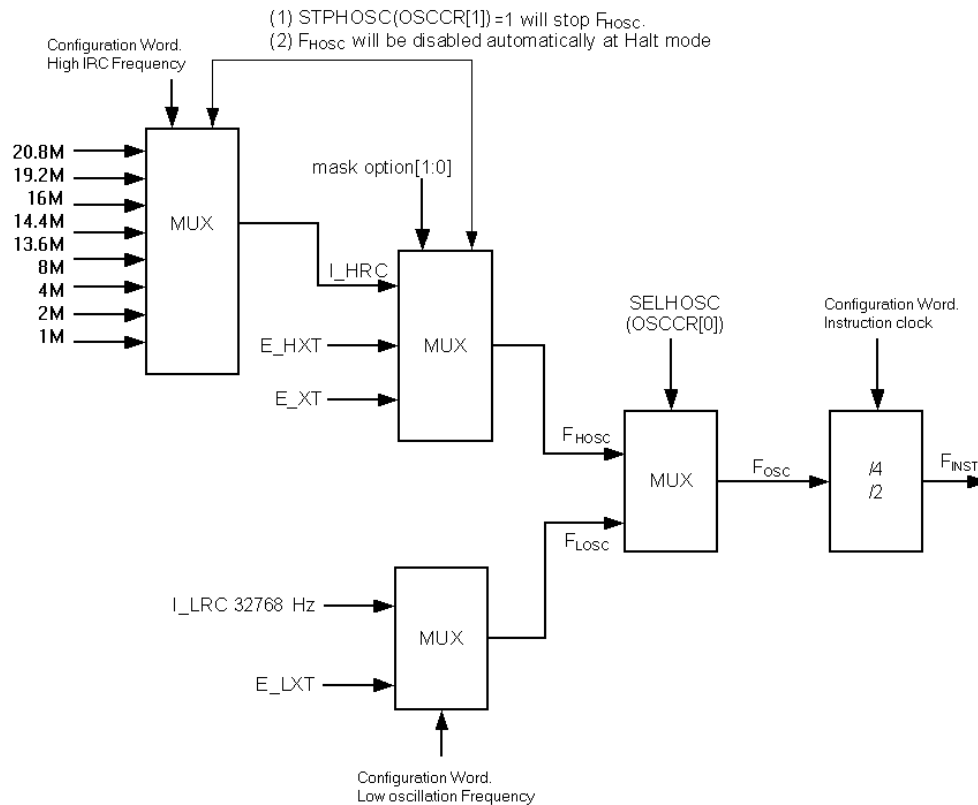
Figure 37 Oscillation Configuration of CY8BE62D
